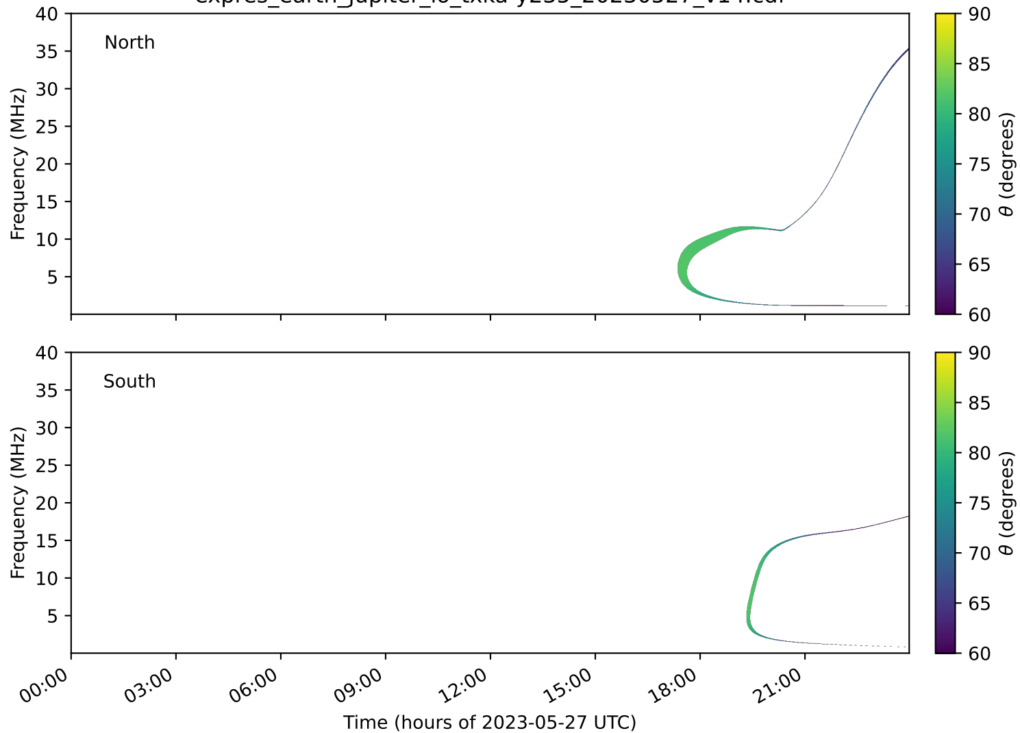
expres_earth_jupiter_io_txka-y235_20230527_v14.cdf
