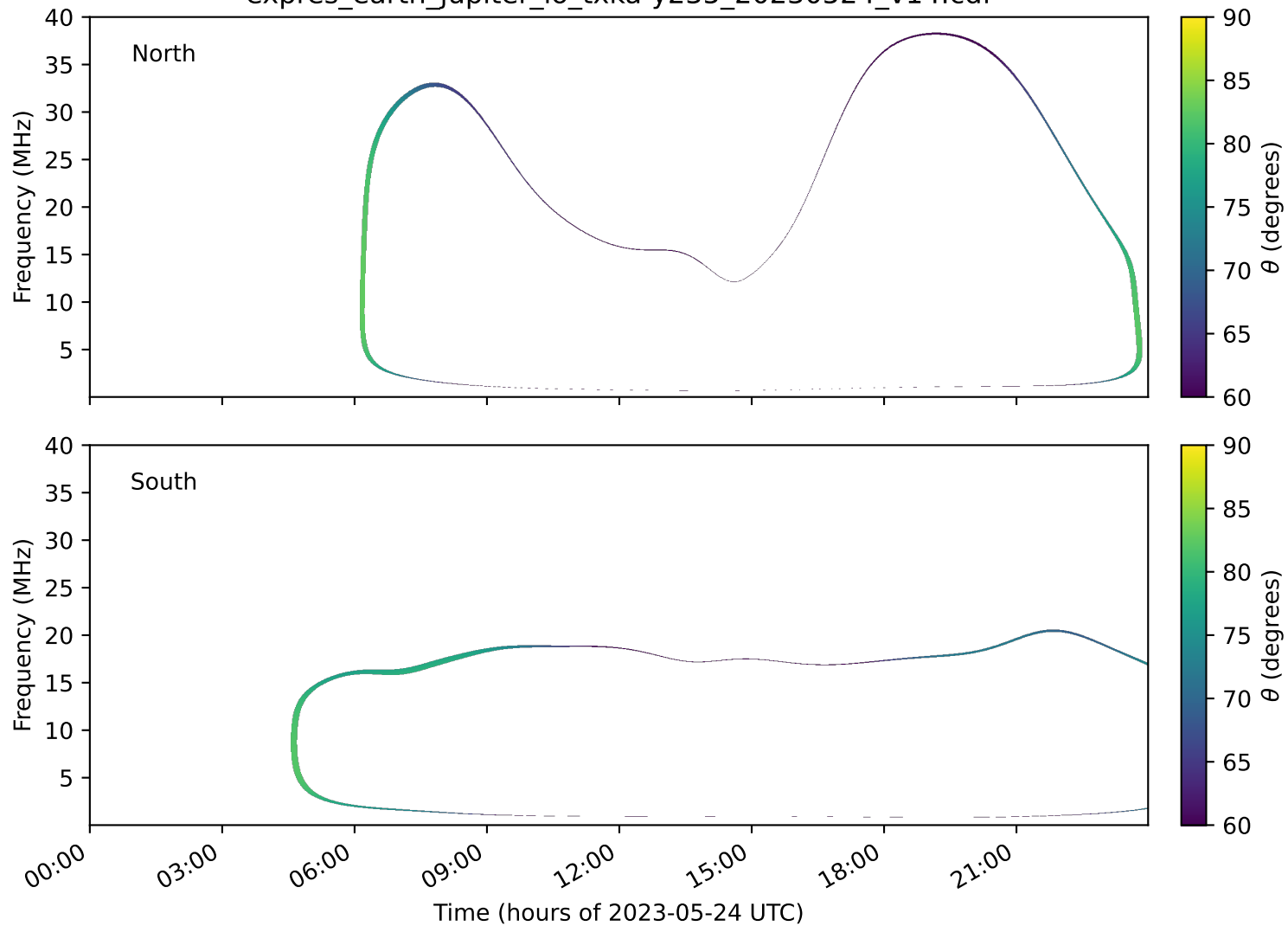
expres_earth_jupiter_io_txka-y235_20230524_v14.cdf
