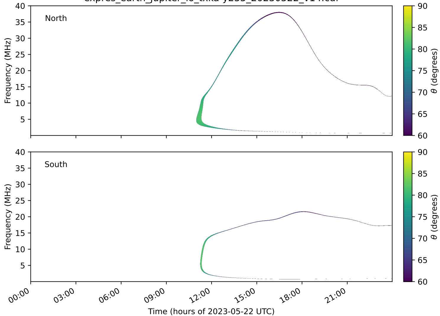
expres_earth_jupiter_io_txka-y235_20230522_v14.cdf
