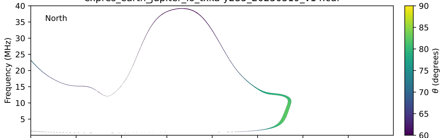
expres_earth_jupiter_io_txka-y235_20230519_v14.cdf
