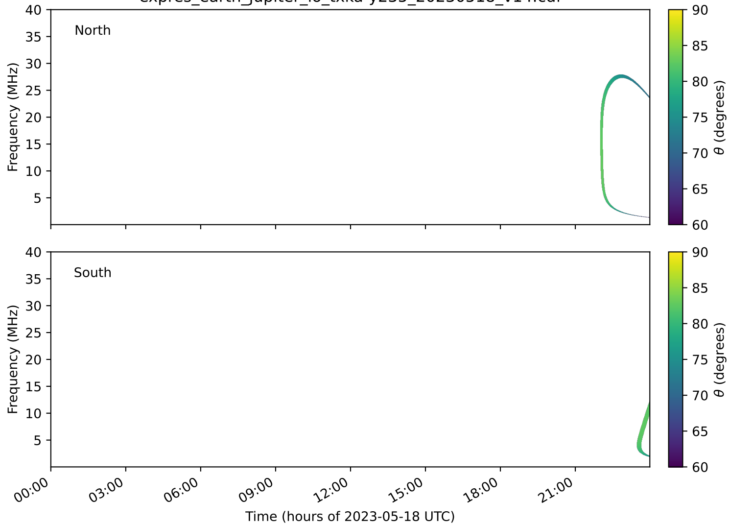
expres_earth_jupiter_io_txka-y235_20230518_v14.cdf
