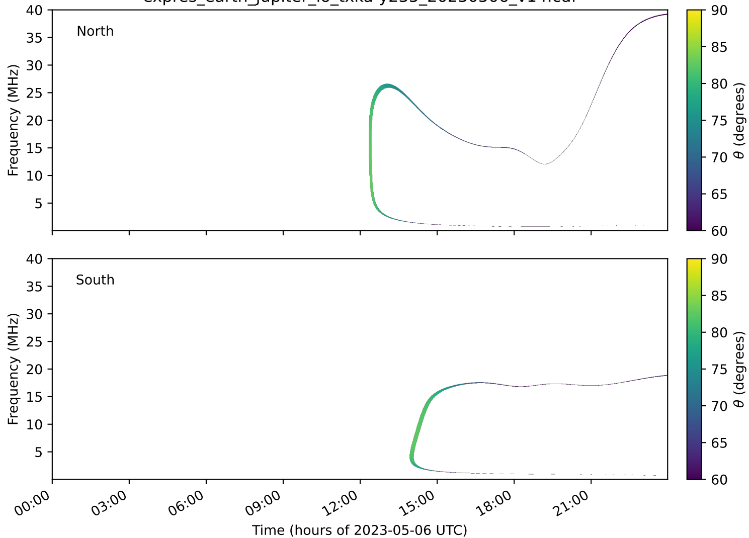
expres_earth_jupiter_io_txka-y235_20230506_v14.cdf
