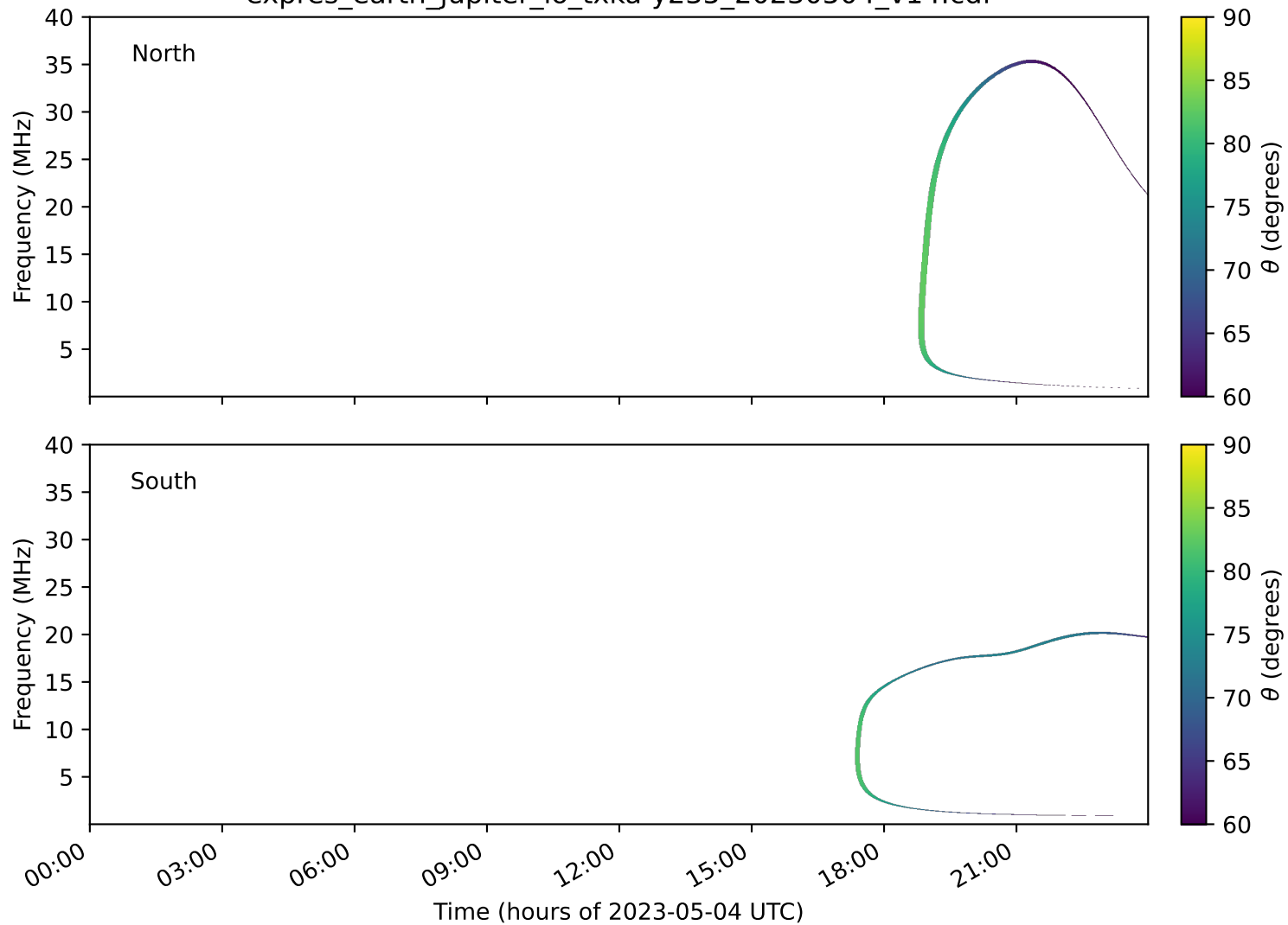
expres_earth_jupiter_io_txka-y235_20230504_v14.cdf
