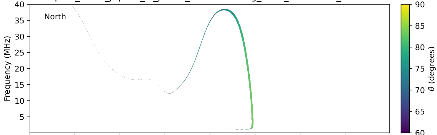
expres_earth_jupiter_io_jrm33_lossc-wid1deg_3kev_20230528_v11.cdf
