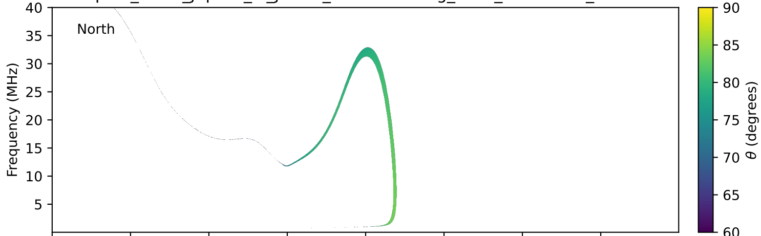
expres_earth_jupiter_io_jrm33_lossc-wid1deg_3kev_20230521_v11.cdf
