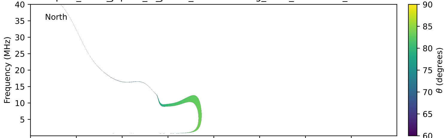
expres_earth_jupiter_io_jrm33_lossc-wid1deg_3kev_20230514_v11.cdf
