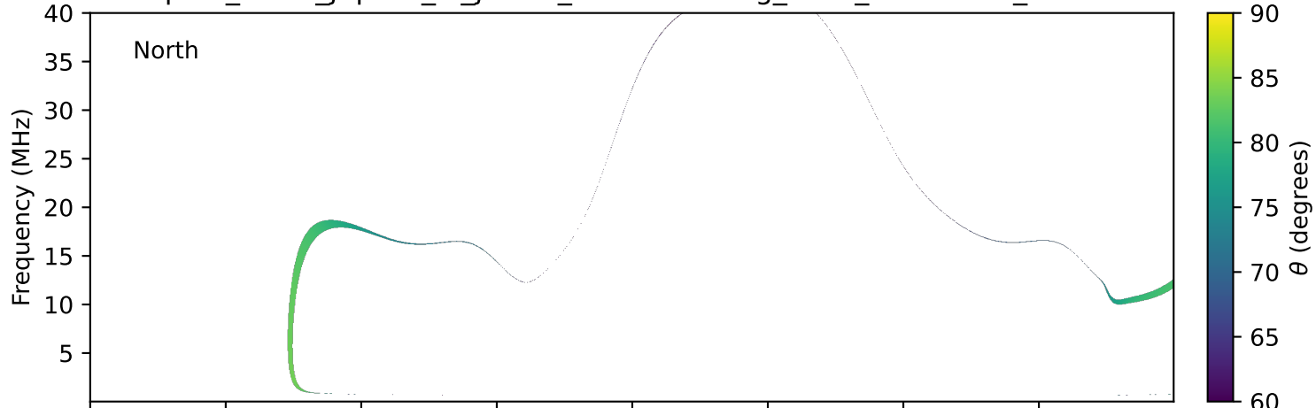
expres_earth_jupiter_io_jrm33_lossc-wid1deg_3kev_20230501_v11.cdf
