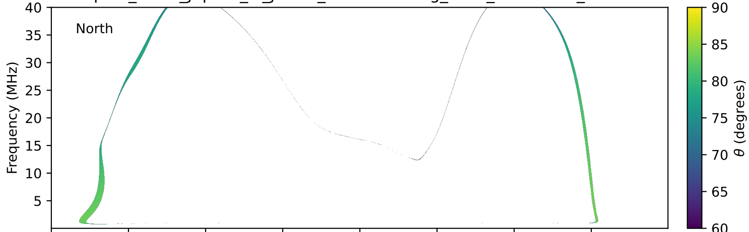
expres_earth_jupiter_io_jrm09_lossc-wid1deg_3kev_20230510_v11.cdf
