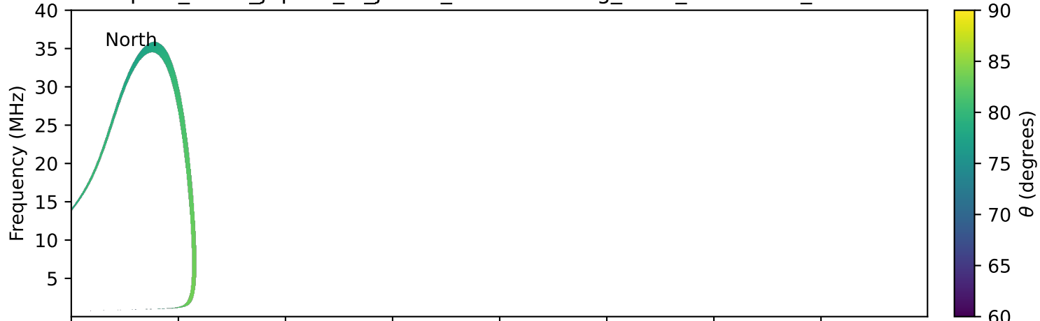
expres_earth_jupiter_io_jrm09_lossc-wid1deg_3kev_20230509_v11.cdf
