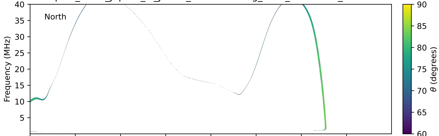
expres_earth_jupiter_io_jrm09_lossc-wid1deg_3kev_20230503_v11.cdf
