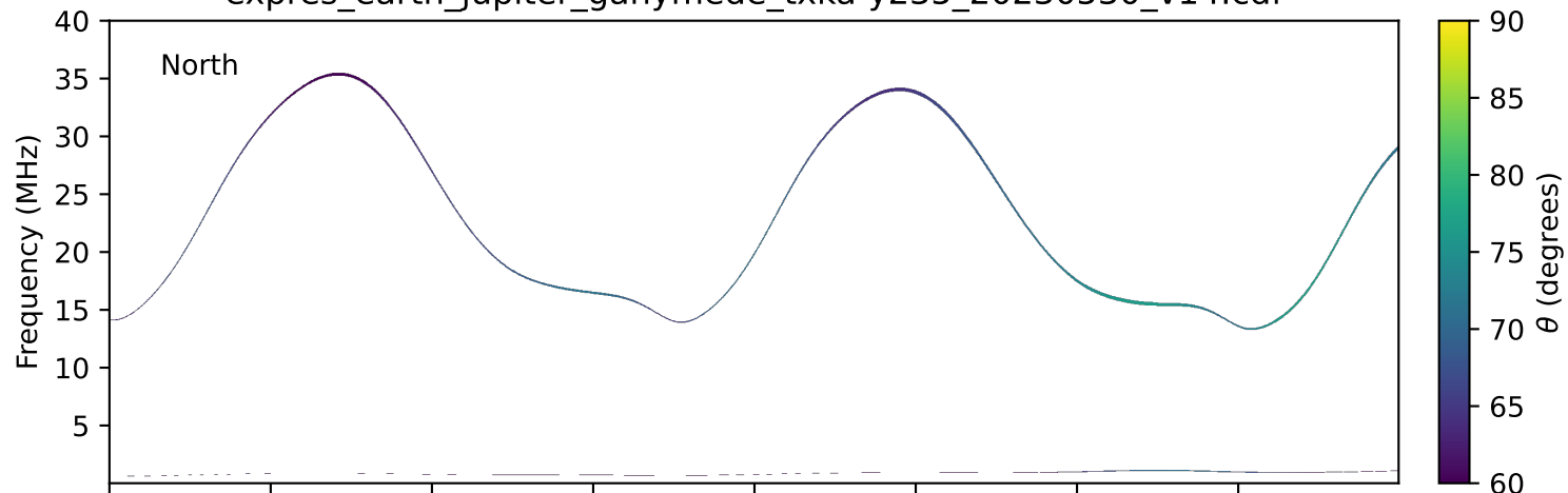
expres_earth_jupiter_ganymede_txka-y235_20230530_v14.cdf
