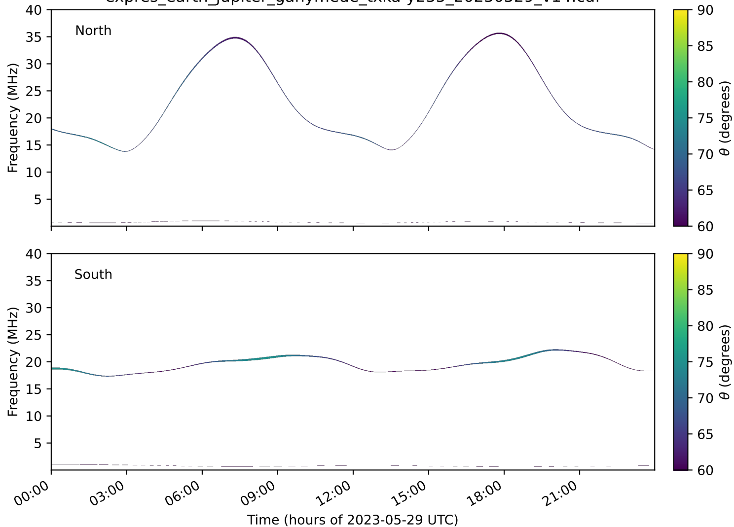
expres_earth_jupiter_ganymede_txka-y235_20230529_v14.cdf
