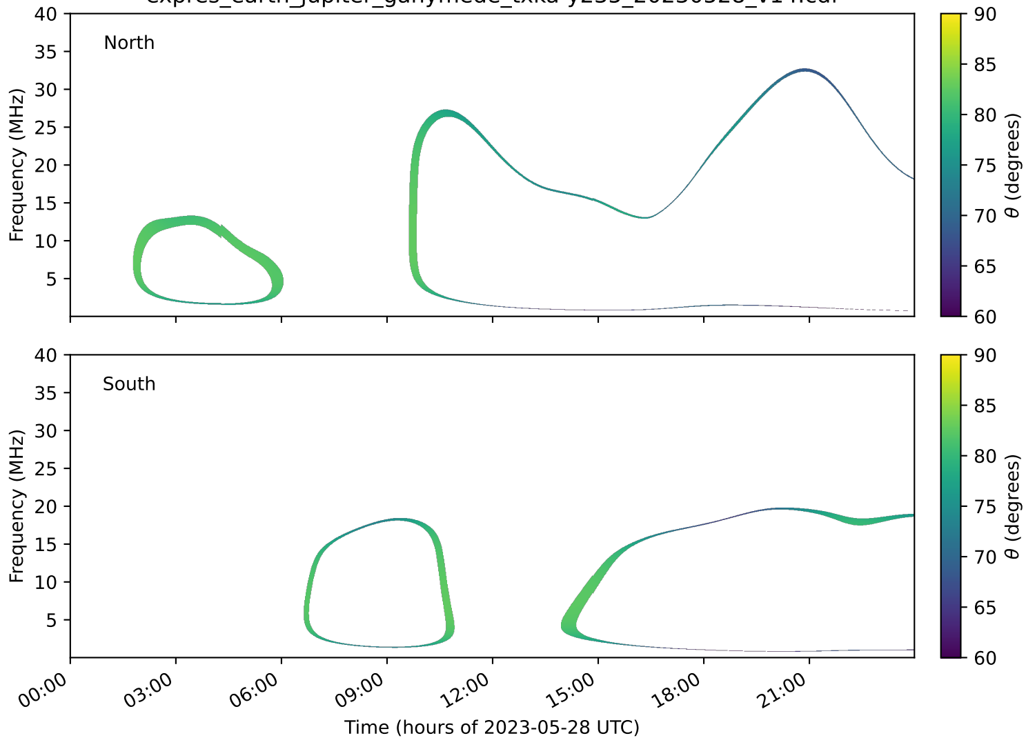
expres_earth_jupiter_ganymede_txka-y235_20230528_v14.cdf
