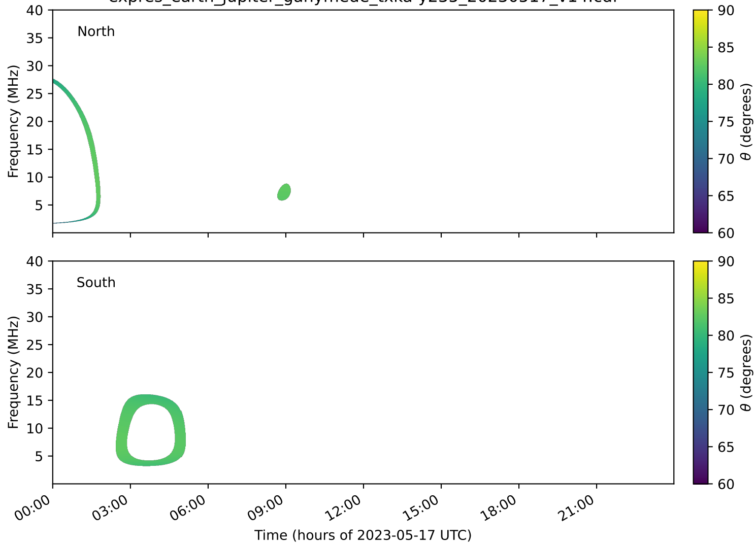
expres_earth_jupiter_ganymede_txka-y235_20230517_v14.cdf
