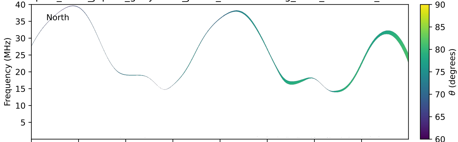
expres_earth_jupiter_ganymede_jrm33_lossc-wid1deg_3kev_20230509_v11.cdf
