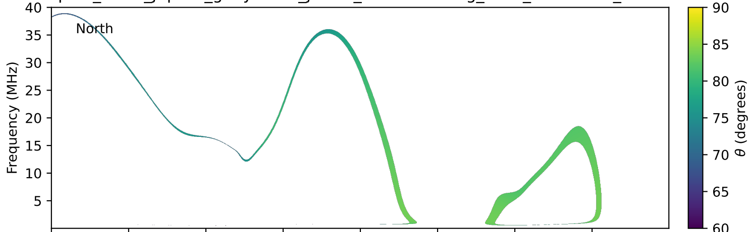
expres_earth_jupiter_ganymede_jrm09_lossc-wid1deg_3kev_20230531_v11.cdf
