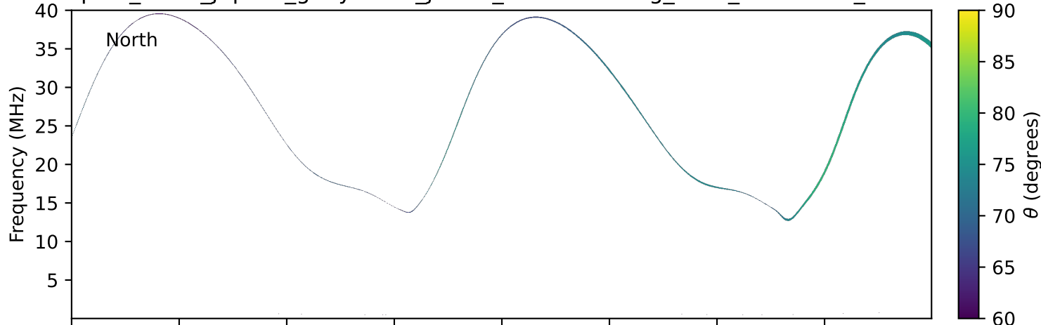
expres_earth_jupiter_ganymede_jrm09_lossc-wid1deg_3kev_20230516_v11.cdf
