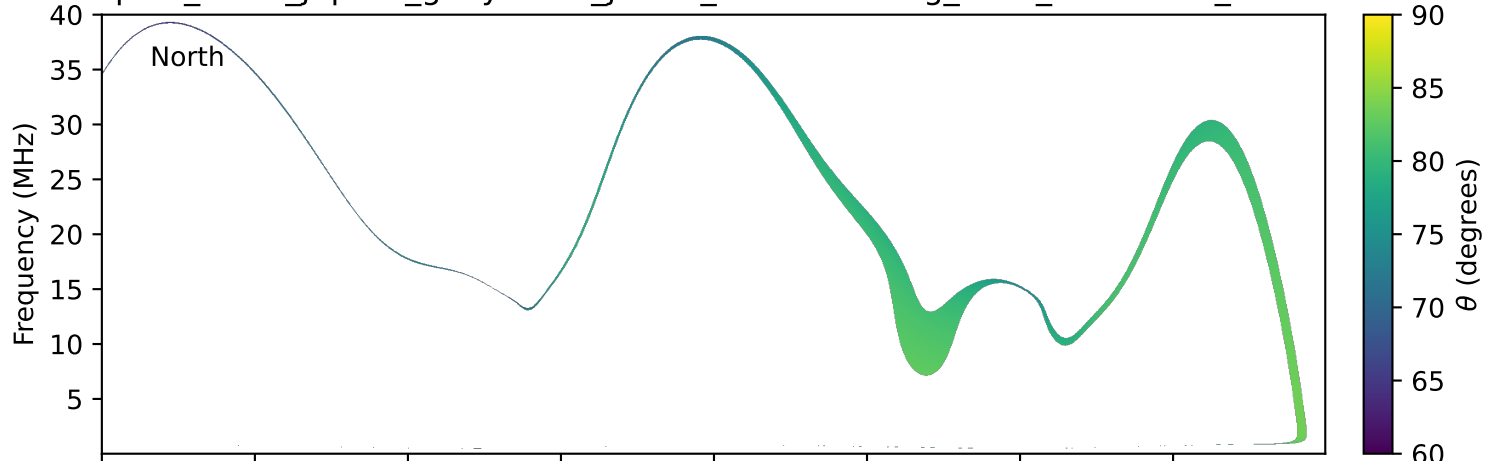
expres_earth_jupiter_ganymede_jrm09_lossc-wid1deg_3kev_20230502_v11.cdf
