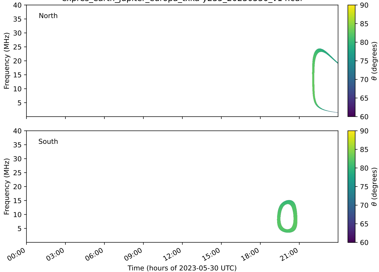
expres_earth_jupiter_europa_txka-y235_20230530_v14.cdf
