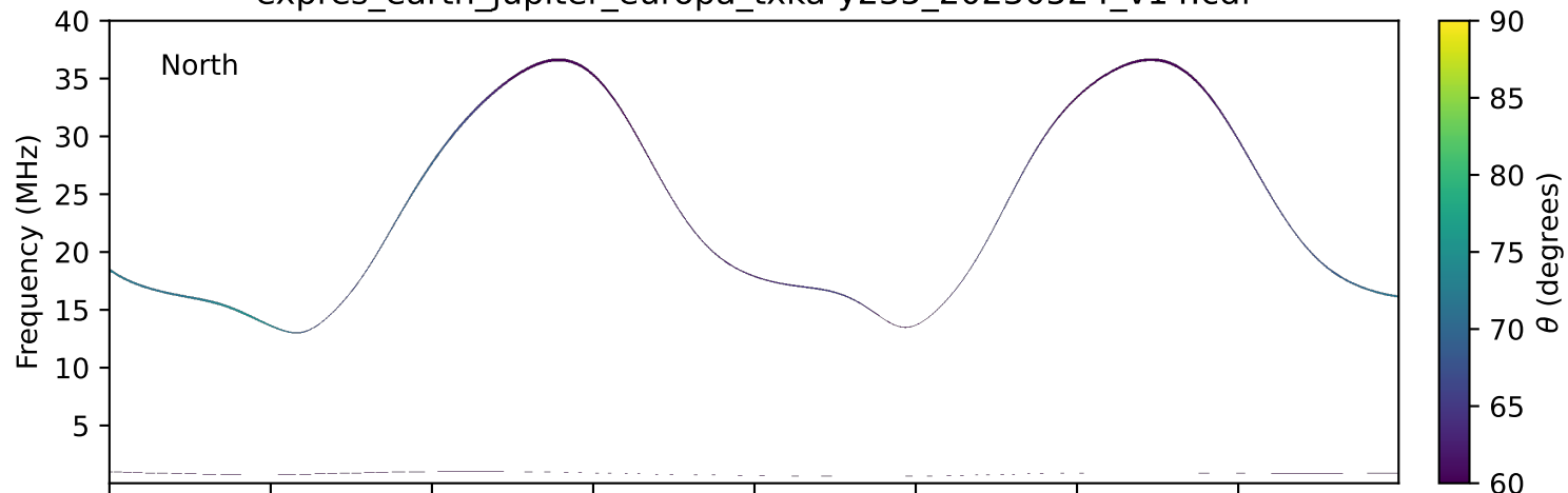
expres_earth_jupiter_europa_txka-y235_20230524_v14.cdf
