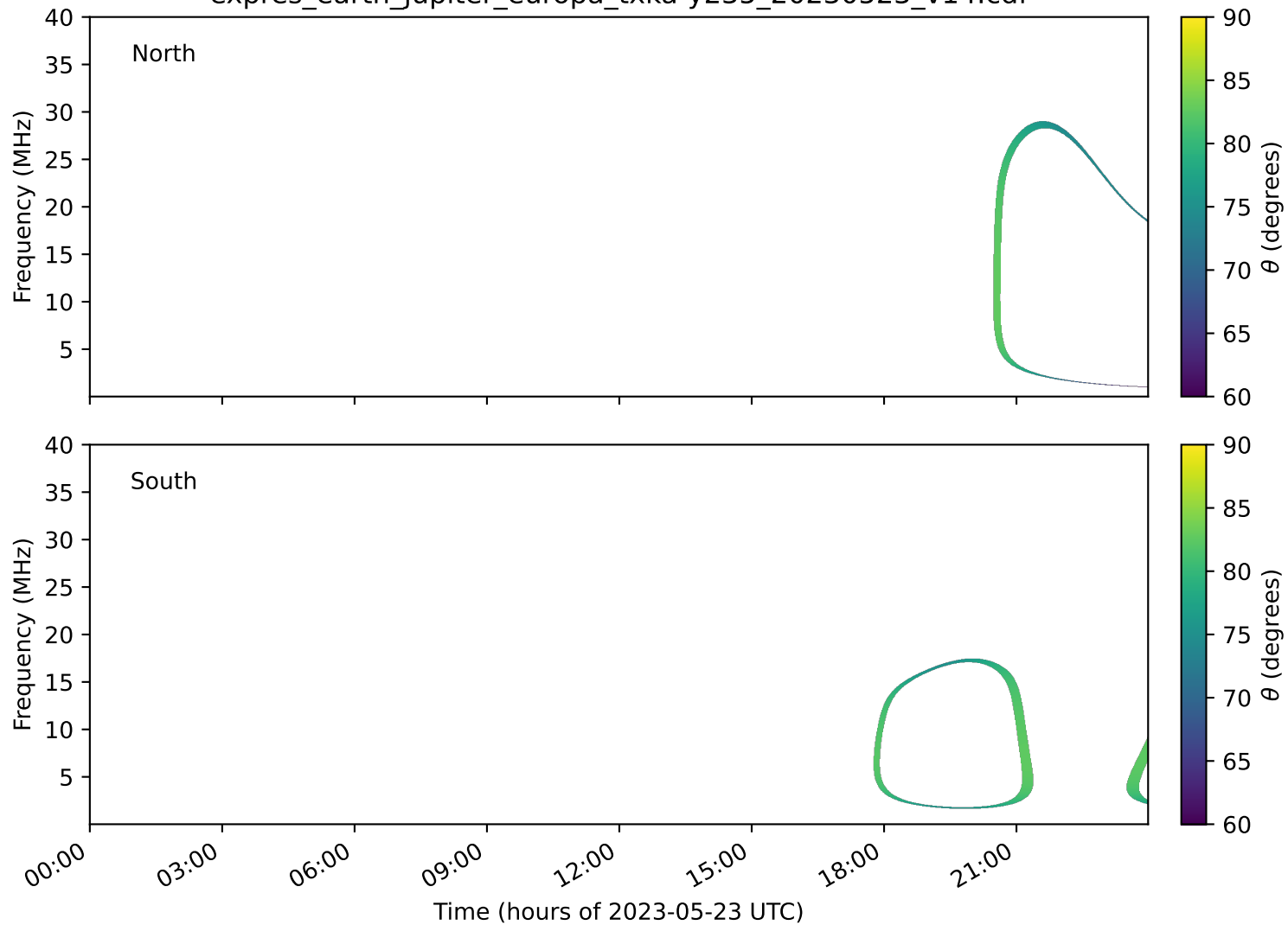
expres_earth_jupiter_europa_txka-y235_20230523_v14.cdf
