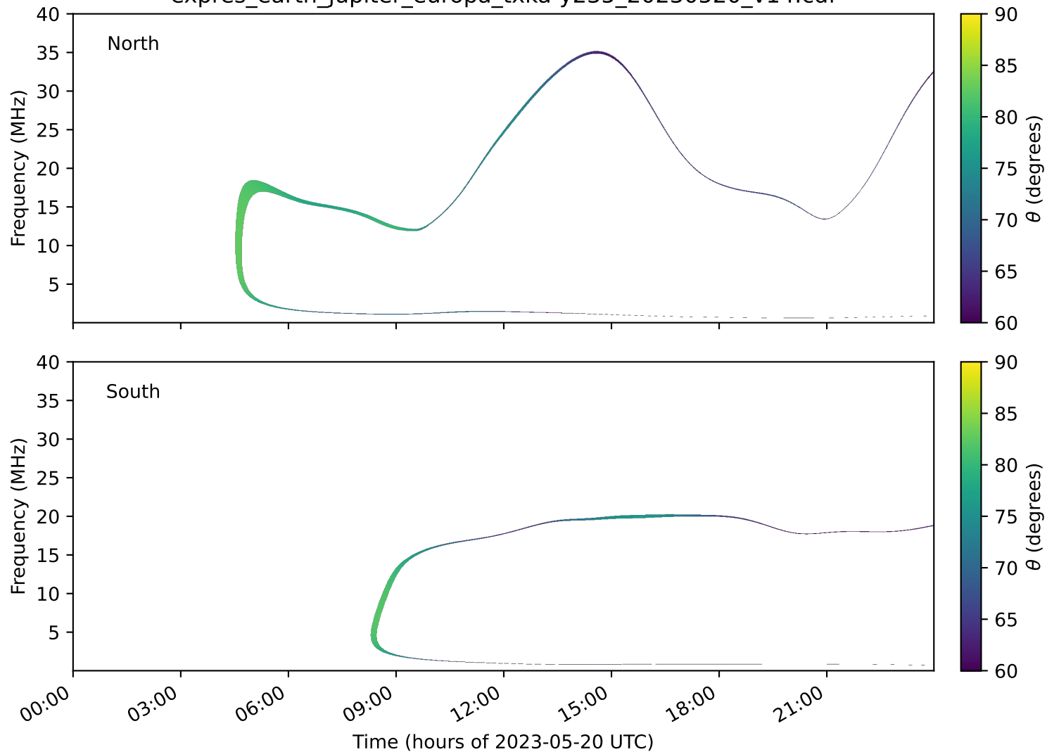
expres_earth_jupiter_europa_txka-y235_20230520_v14.cdf
