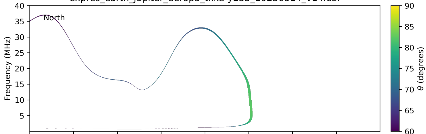
expres_earth_jupiter_europa_txka-y235_20230514_v14.cdf
