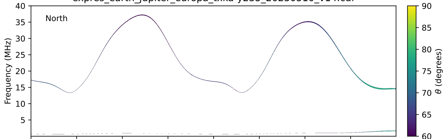
expres_earth_jupiter_europa_txka-y235_20230510_v14.cdf
