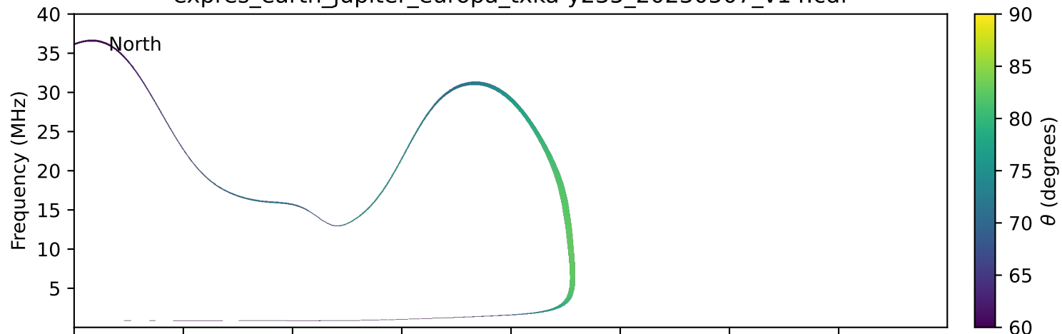
expres_earth_jupiter_europa_txka-y235_20230507_v14.cdf
