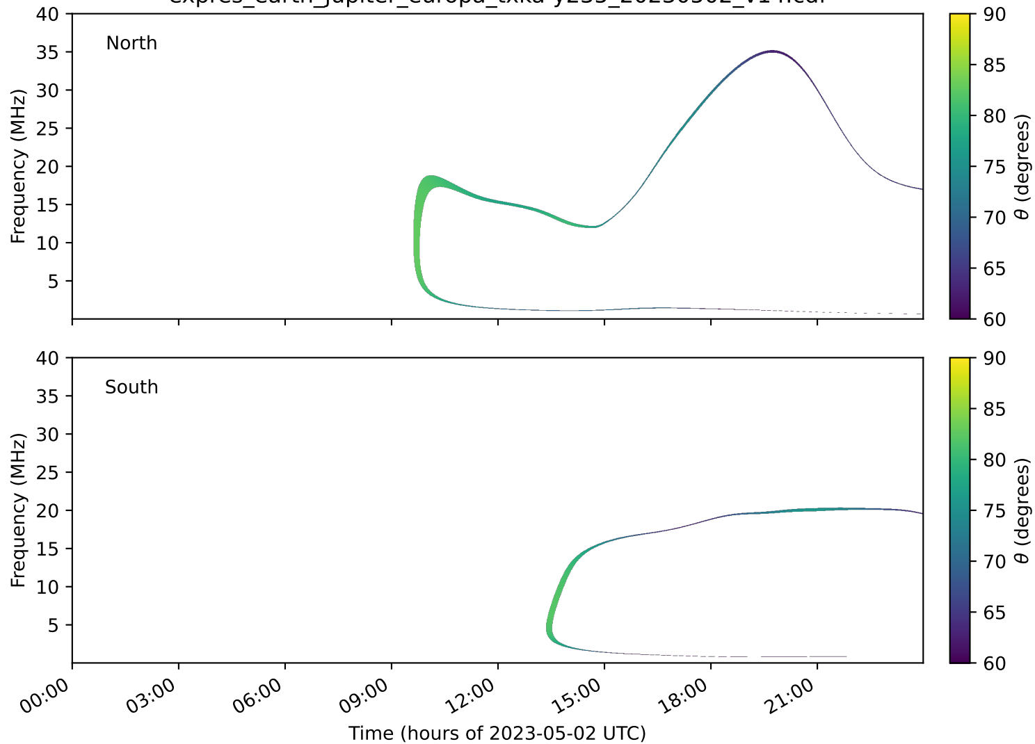
expres_earth_jupiter_europa_txka-y235_20230502_v14.cdf
