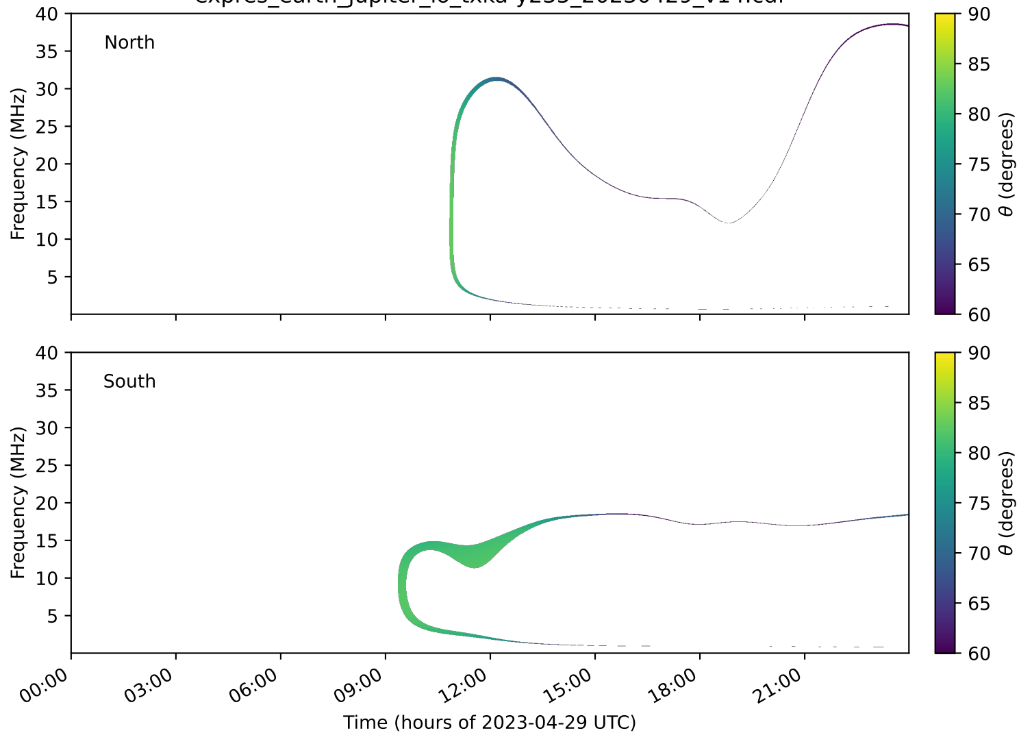
expres_earth_jupiter_io_txka-y235_20230429_v14.cdf
