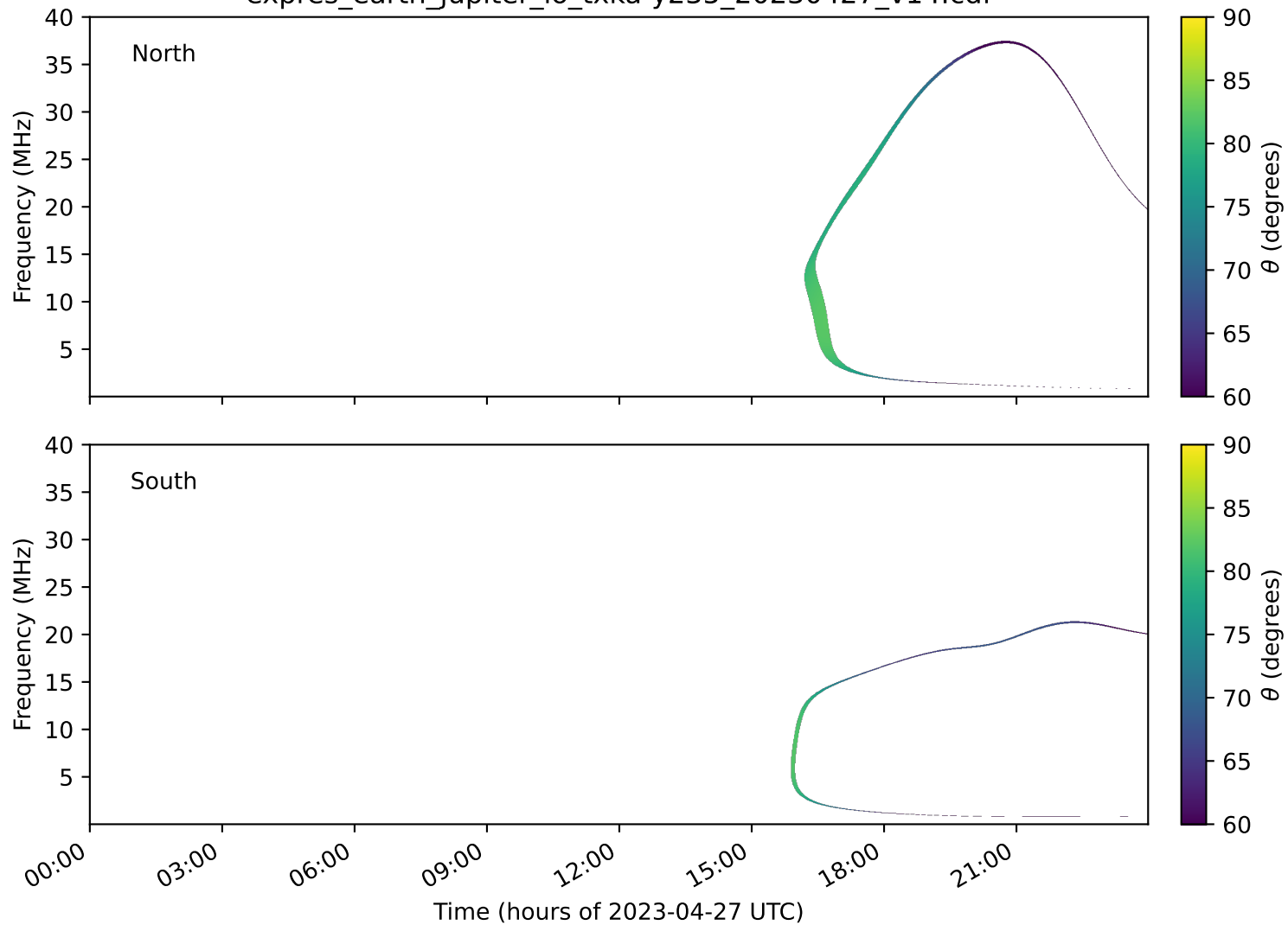
expres_earth_jupiter_io_txka-y235_20230427_v14.cdf
