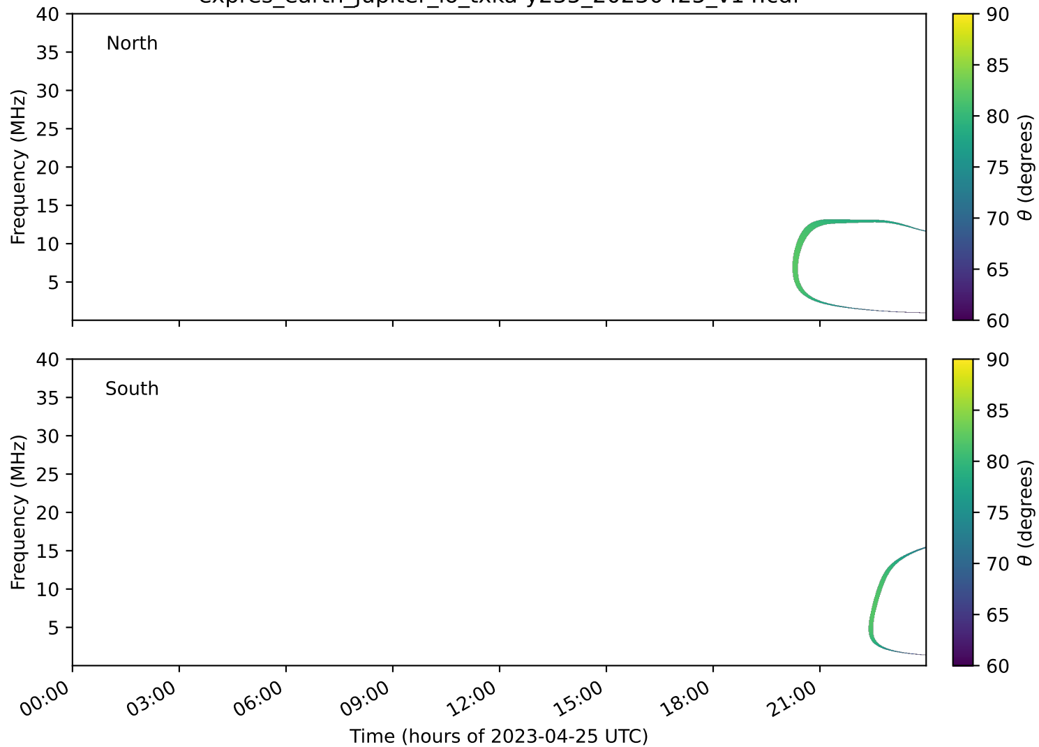
expres_earth_jupiter_io_txka-y235_20230425_v14.cdf
