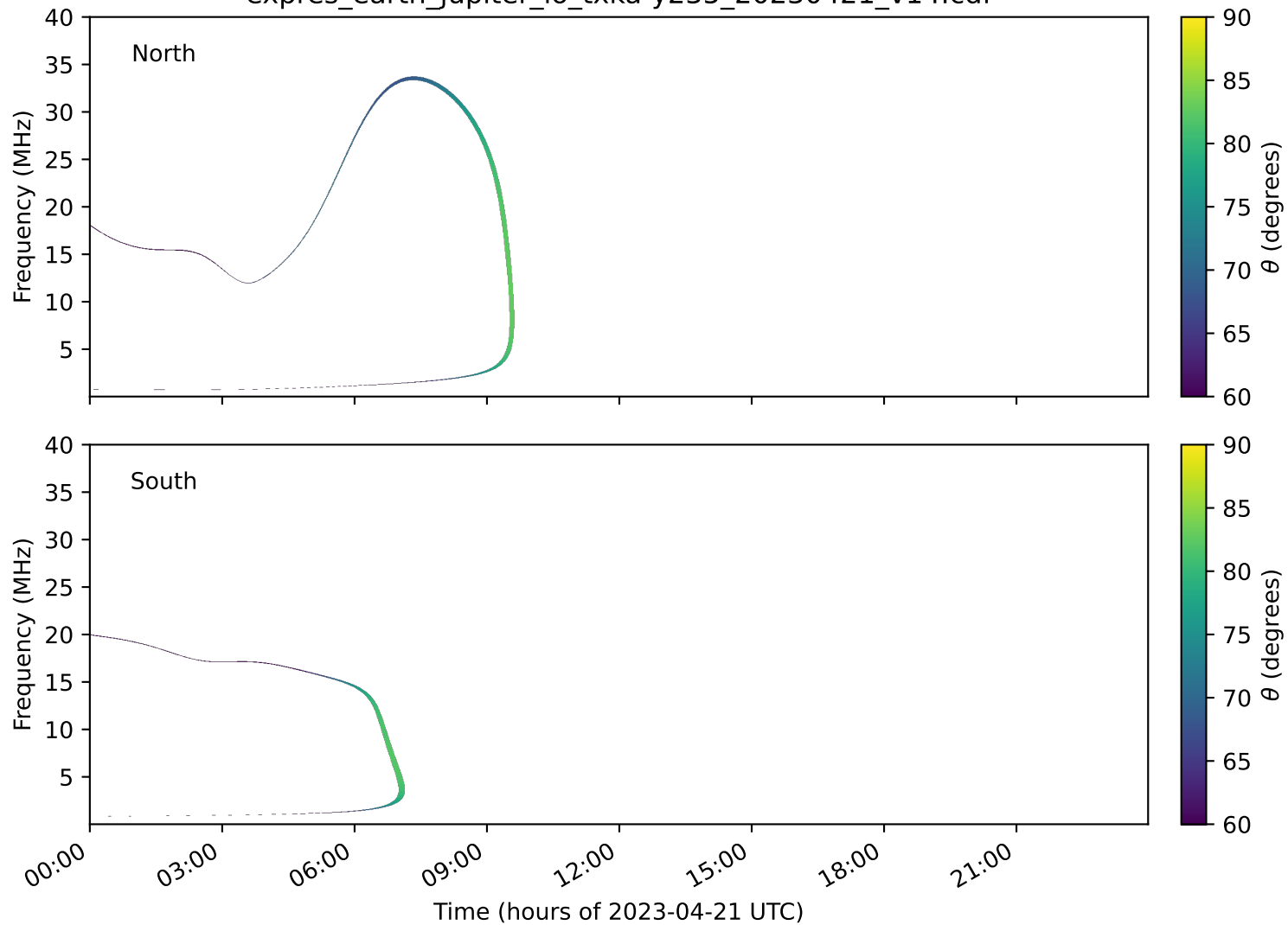
expres_earth_jupiter_io_txka-y235_20230421_v14.cdf
