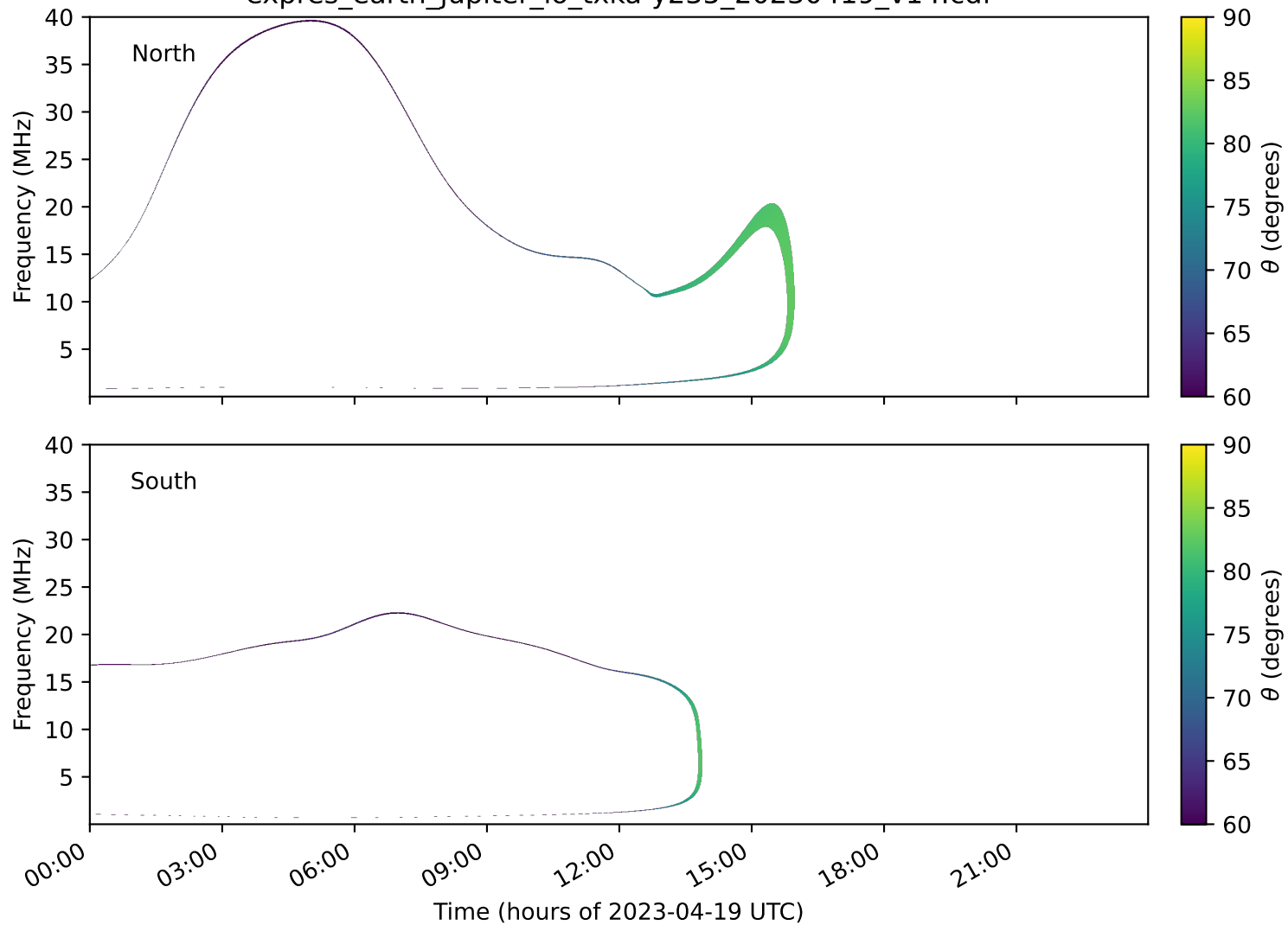
expres_earth_jupiter_io_txka-y235_20230419_v14.cdf
