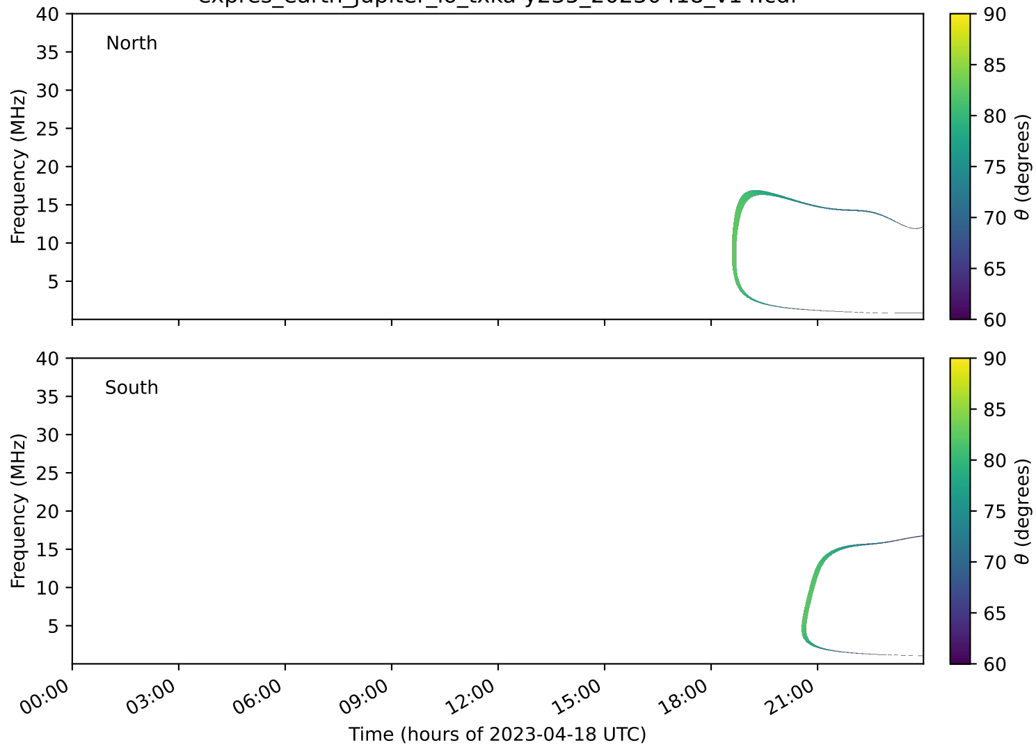
expres_earth_jupiter_io_txka-y235_20230418_v14.cdf
