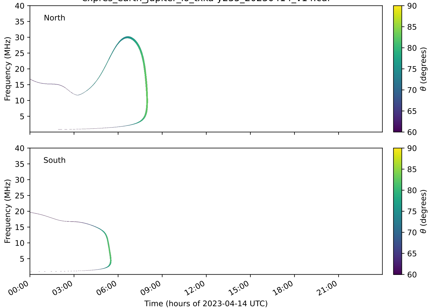
expres_earth_jupiter_io_txka-y235_20230414_v14.cdf
