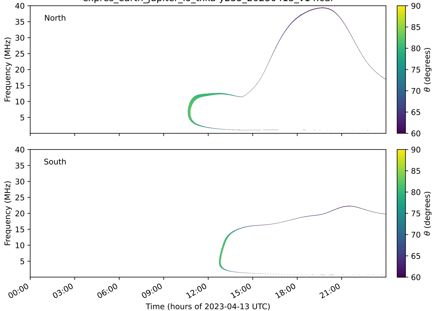
expres_earth_jupiter_io_txka-y235_20230413_v14.cdf
