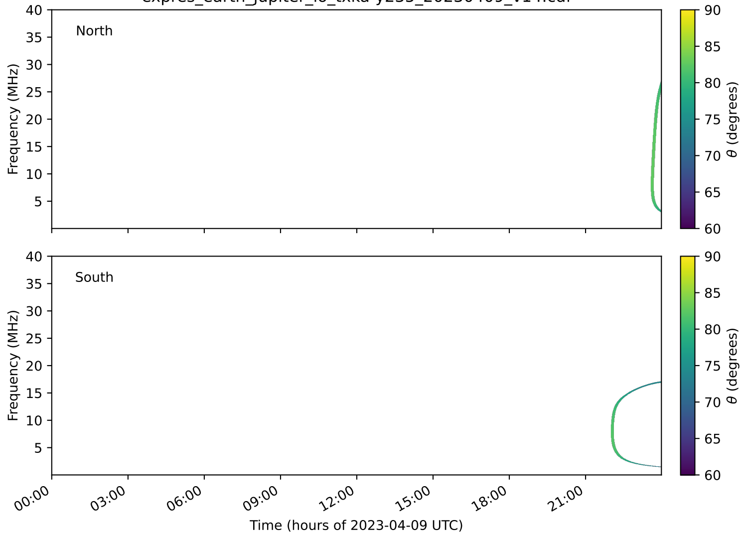
expres_earth_jupiter_io_txka-y235_20230409_v14.cdf
