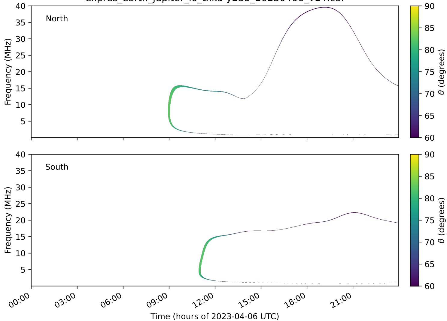
expres_earth_jupiter_io_txka-y235_20230406_v14.cdf
