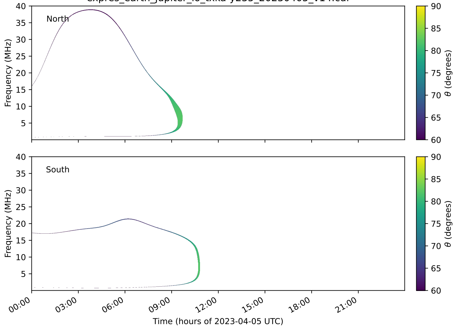
expres_earth_jupiter_io_txka-y235_20230405_v14.cdf
