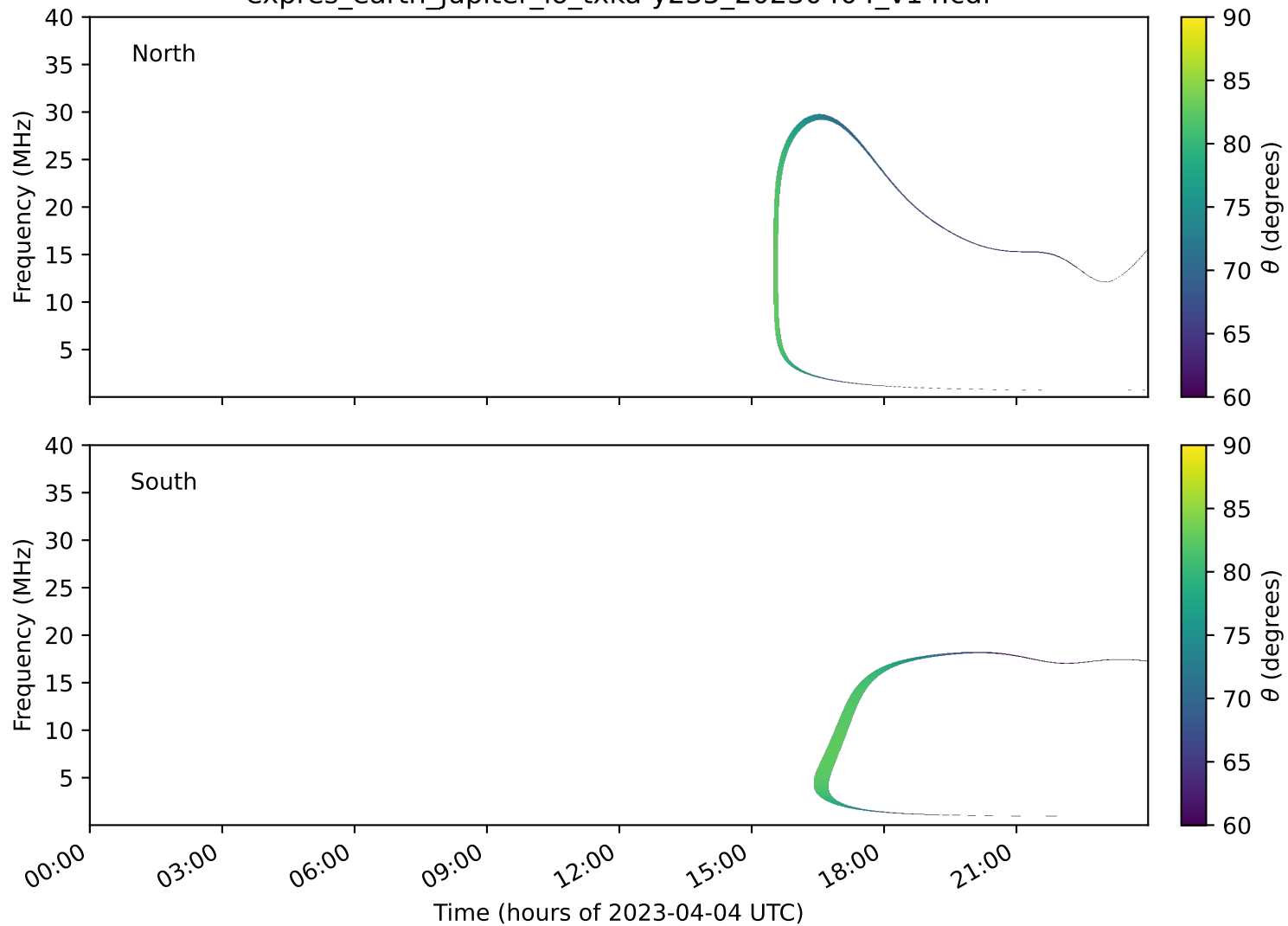
expres_earth_jupiter_io_txka-y235_20230404_v14.cdf
