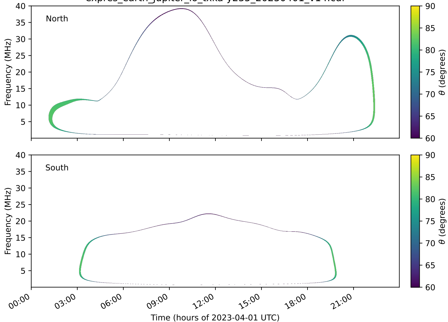
expres_earth_jupiter_io_txka-y235_20230401_v14.cdf
