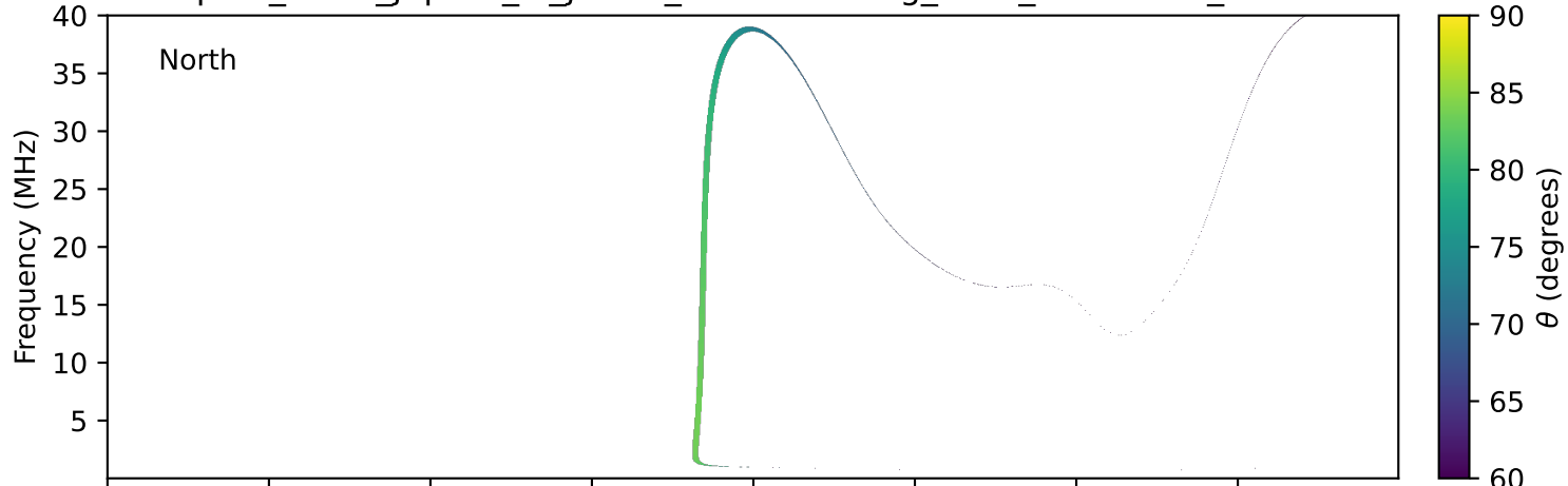
expres_earth_jupiter_io_jrm33_lossc-wid1deg_3kev_20230429_v11.cdf
