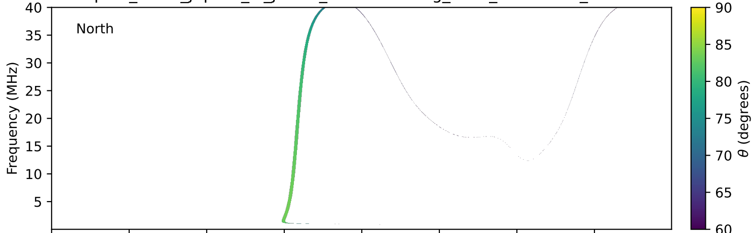
expres_earth_jupiter_io_jrm33_lossc-wid1deg_3kev_20230422_v11.cdf
