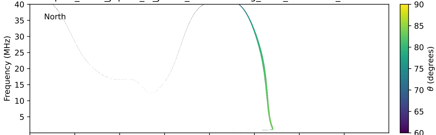
expres_earth_jupiter_io_jrm33_lossc-wid1deg_3kev_20230403_v11.cdf
