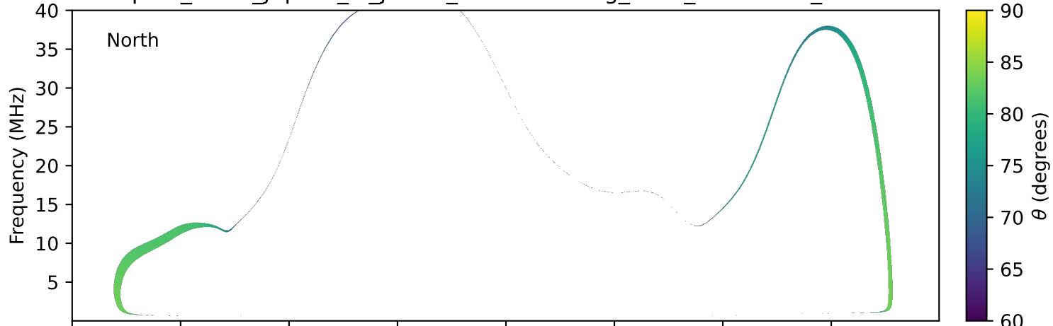
expres_earth_jupiter_io_jrm33_lossc-wid1deg_3kev_20230401_v11.cdf
