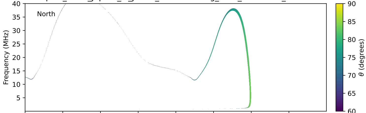
expres_earth_jupiter_io_jrm09_lossc-wid1deg_3kev_20230426_v11.cdf
