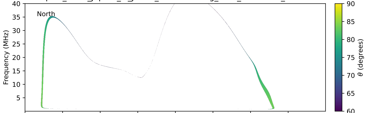
expres_earth_jupiter_io_jrm09_lossc-wid1deg_3kev_20230417_v11.cdf
