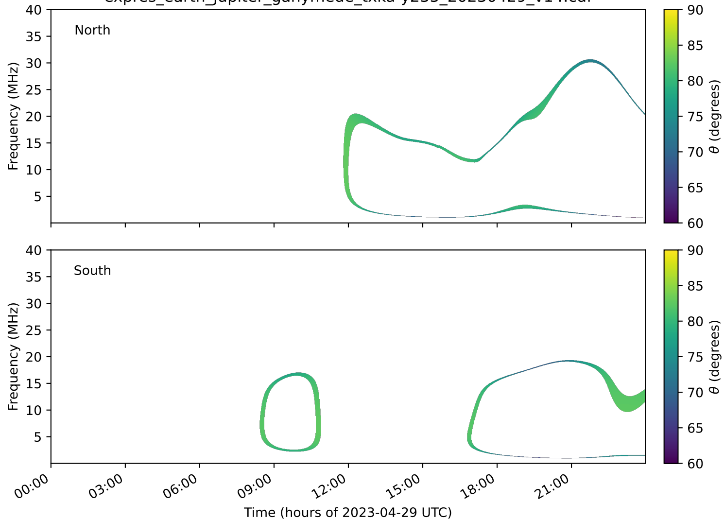
expres_earth_jupiter_ganymede_txka-y235_20230429_v14.cdf
